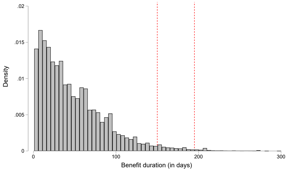
FIGURE A1 — Density of UI Benefit Duration Length, in Days
